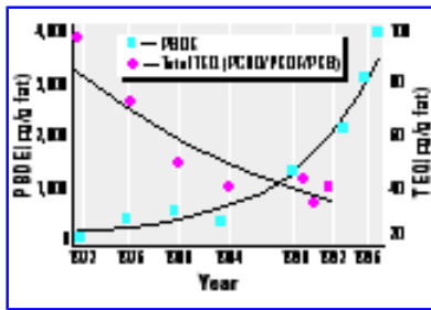
Figure 1. Organohalogen compounds in human milk in Sweden. Abbreviations: PCDD, polychlorinated dibenzo- p -dioxin; PCDF, polychlorinated dibenzofuran; PCB, polychlorinated biphenyl; TEQ, toxic equivalent. Adapted from Norén and Mieronytė (1).
