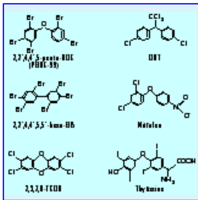
Figure 2. Examples of polybrominated diphenyl ethers and structurally related compounds. Abbreviations: hexa-BB, hexabromobiphenyl; penta-BDE, pentabromodiphenyl ether; TCDD, tetrachlorodibenzo- p -dioxin.
